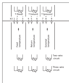
Terminal diagram, PT 100 temperature board
