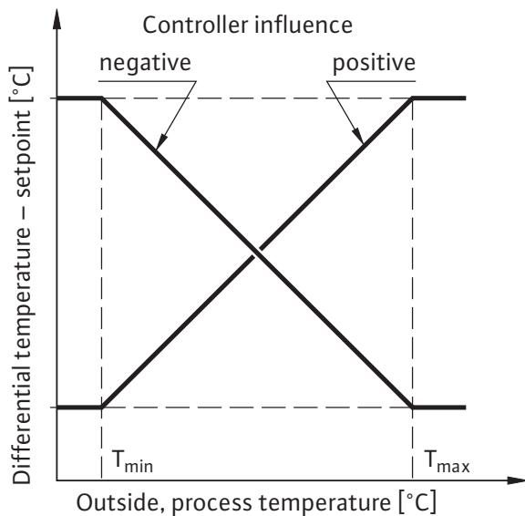
Fig.: Effect on the differential temperature
