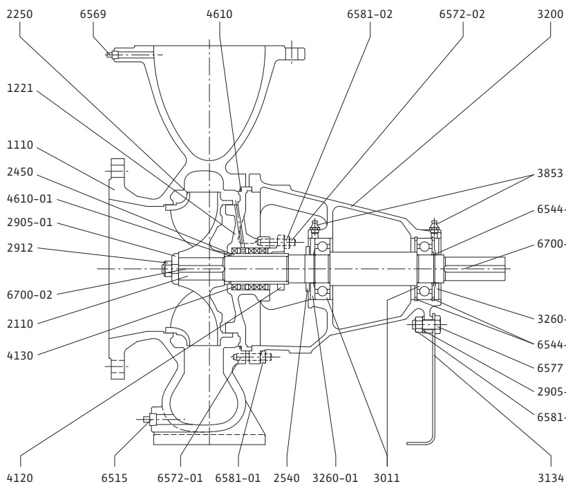
Cross-sectional drawing: Pump with bearing B3 (version with stuffing box)
