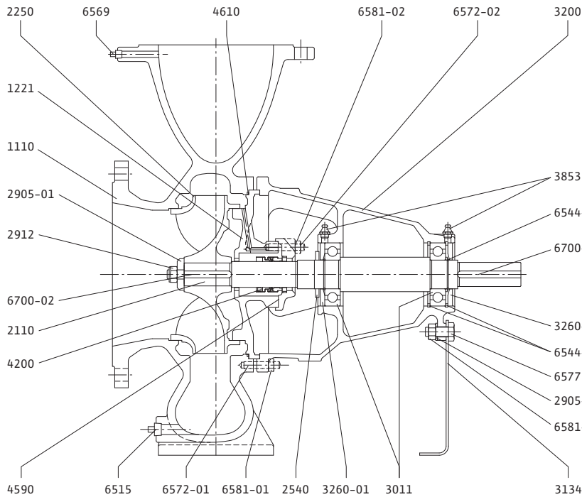
Cross-section drawing: Pump with bearing B3 (version with mechanical seal)
