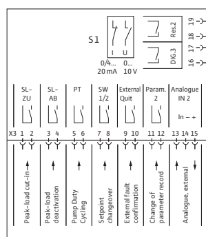
Terminal diagram, DDC board
