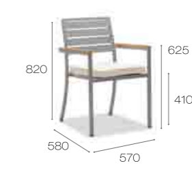
Dining Arm Chair _ 657611 Shown at: P 252-253
