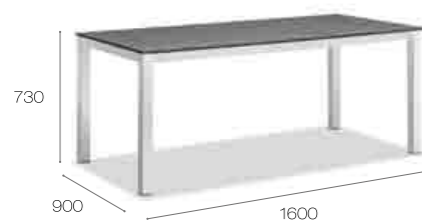
Rectangular Dining Table_ 647771 Shown at: P 294-295
