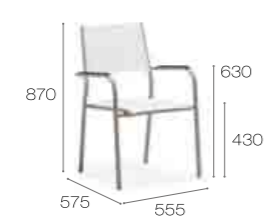
Dining Arm Chair _ 660111 Shown at: P 244-245
