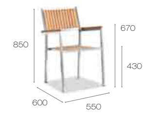
Dining Arm Chair _ 800111 Shown at: P 210-211
